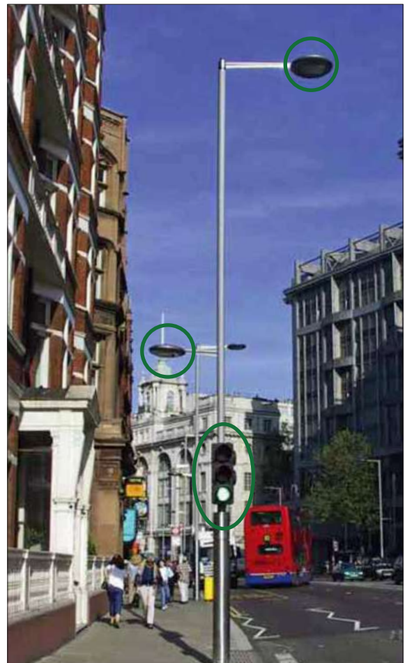
Figure 4.22: Example of a light installation that is designed with both the pedestrian and the vehicle in mind and also incorporates signals for a pedestrian crossing (image source: Camden Streetscape Manual).
